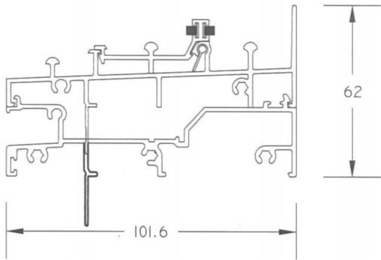
QUANTUM SLIDING DOOR SILL WITH SUMPSILL
